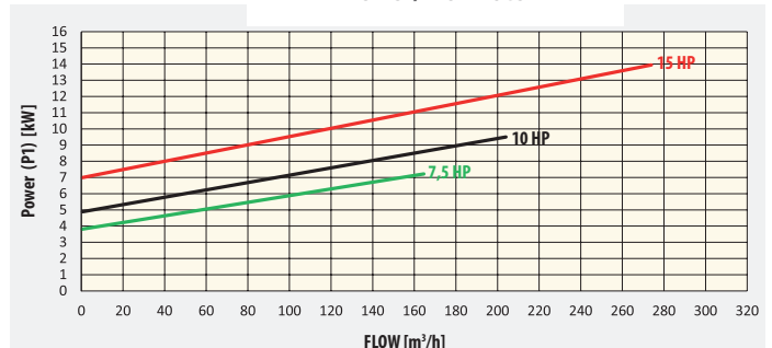
Power/Flow rate
