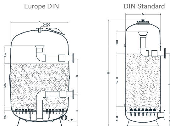
Monolayer - Outlet water above nozzle plate for European DIN.
