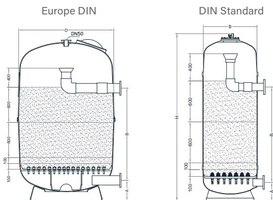
Multilayer - Outlet water under nozzle plate.
