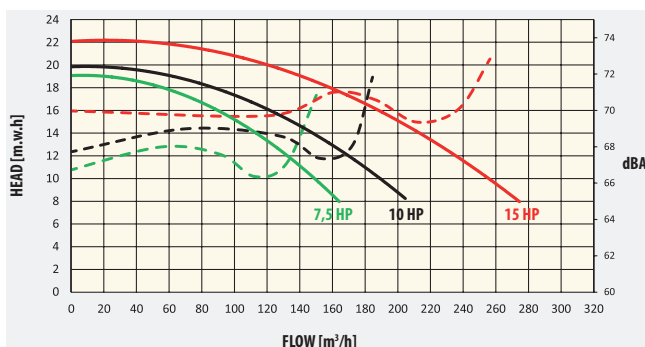
Pressure/Flow rate
