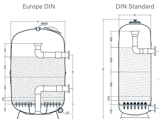
Multilayer - Outlet water above nozzle plate for European DIN.
