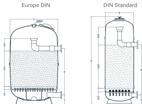
Monolayer - Outlet water under nozzle plate.
