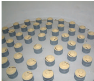
Nozzle plate detail
